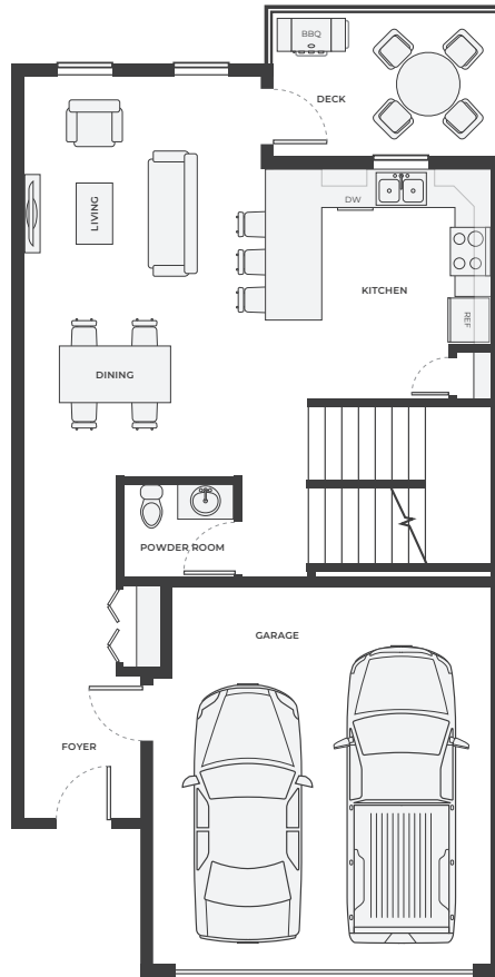
MAIN FLOOR 1,170 SQ.FT.
