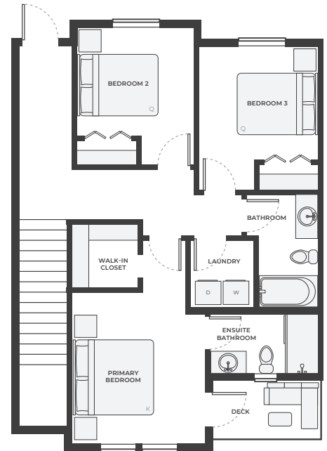
TOP FLOOR
